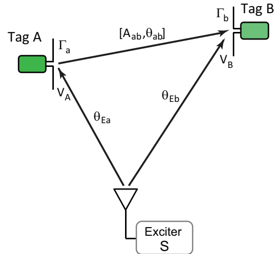
Fig. 1. Tag-to-tag channel.
