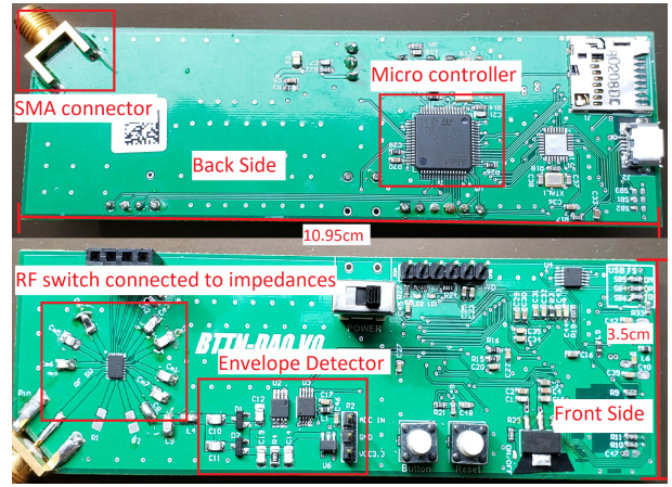
Fig. 2. Discrete implementation of RF tag used in experiments.
