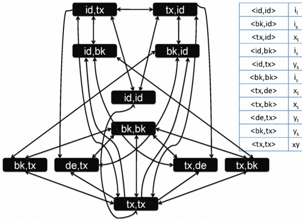
Figure 2. Markov model of the combined MAC Layer behavior of two nodes (sender side only). Note that some arrows are bidirectional.
