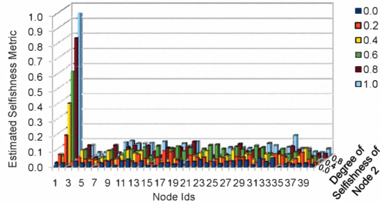
Figure 4. Simulation results for a 40 node network. Node 2 is the only selfish node. The estimated selfishness metric using heuristic H_2 is shown for each node for each of the 6 sets of simulations that are run with different degree of selfishness of node 2.
