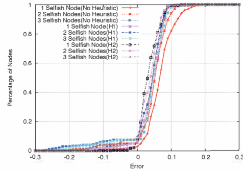
Figure 5. CDF of 'estimation error' for the selfishness metric. Three different scenarios are presented where number of selfish nodes are varied (1, 2 or 3) and witness nodes are identified in three different ways.
