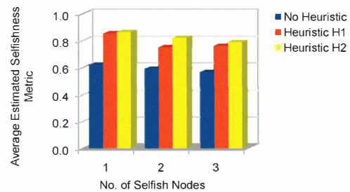
Figure 6. Simulation results for the sparse network.
