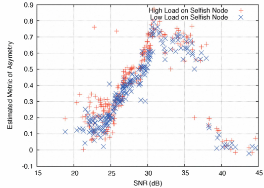
Figure 3. Experimental results with varying load on the selfish node.
